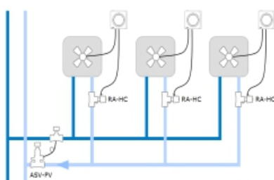
Example of GreenCon RC-T2 used in 2 pipe fan coil unit application.
