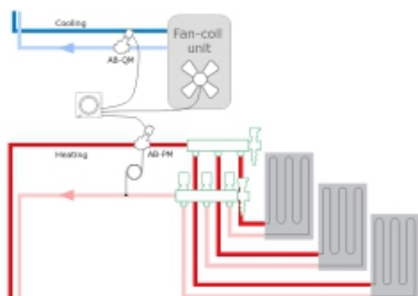
Example of GreenCon RC-T4 used in combined floor heating/FCU cooling application.
